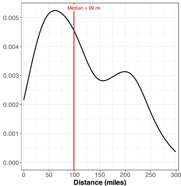
Figure 2: Distance Distribution
